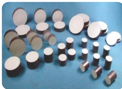
ZnO Element
