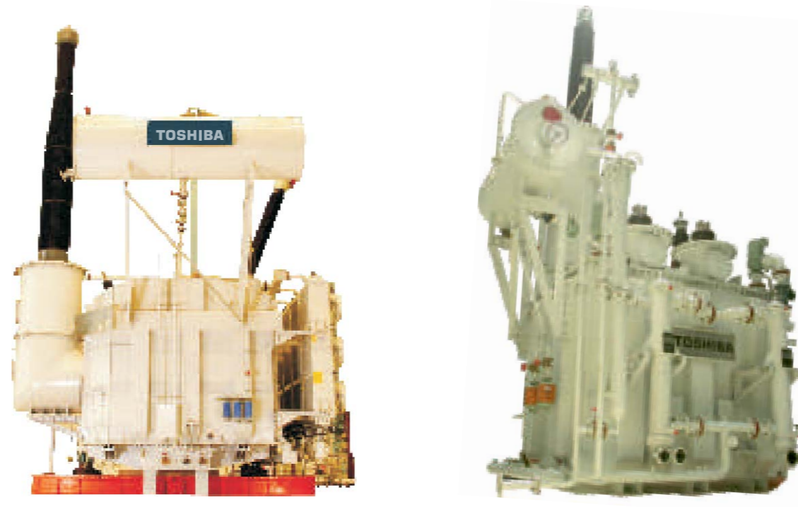
Upto 1500 MVA, 1200kV
