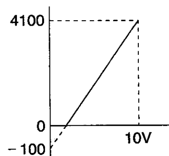
After offset correction
