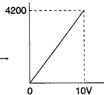
After gain correction
