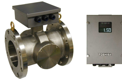
Figure 2. LQ500 Density (consistency) Meter
