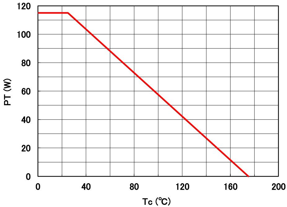
Power Dissipation vs. Case Temperature
