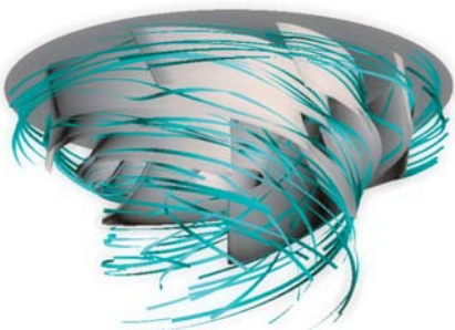
Flow analysis of the splitter runner
