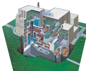
Advanced BWR (ABWR)
