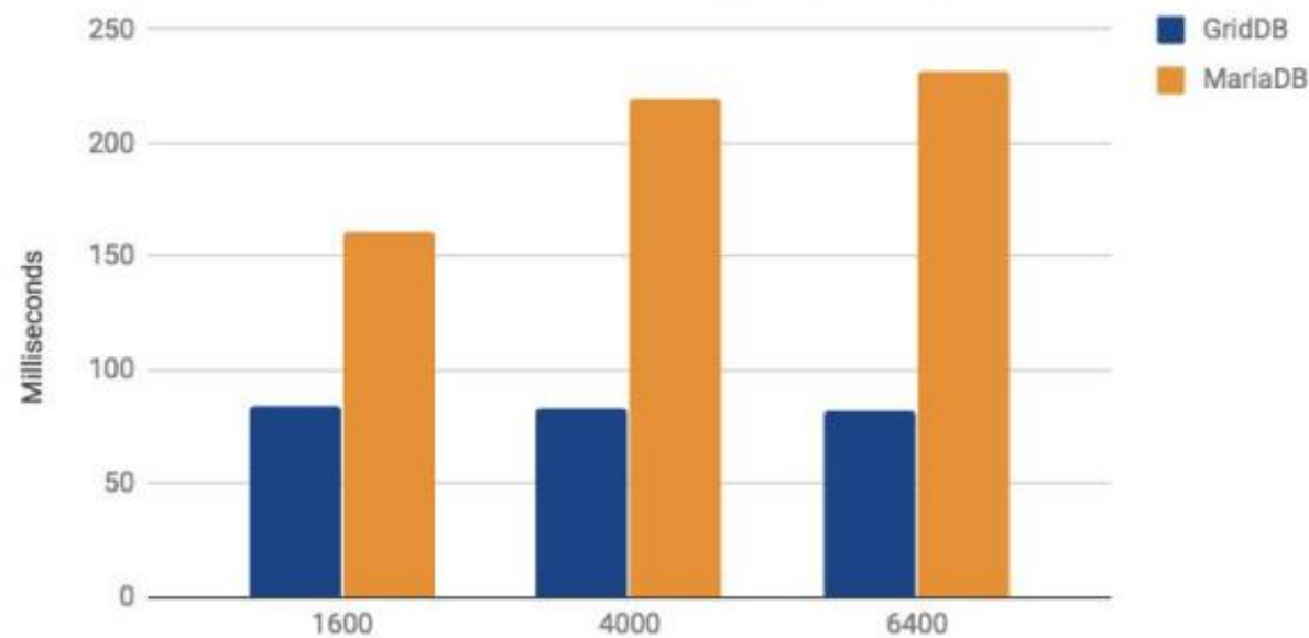
Average Milliseconds Per Billing Aggregation (Fewer is better)
